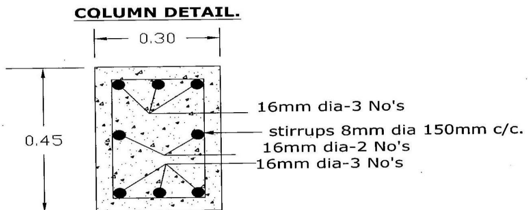
X- SECTION AT END
