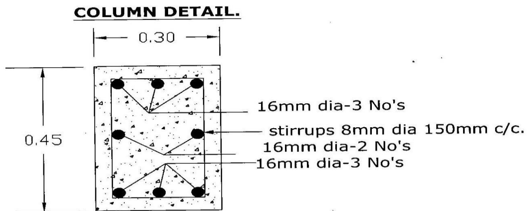
X- SECTION AT CENTRE
