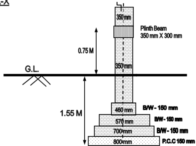
DETAIL OF WALL FOUNDATION
