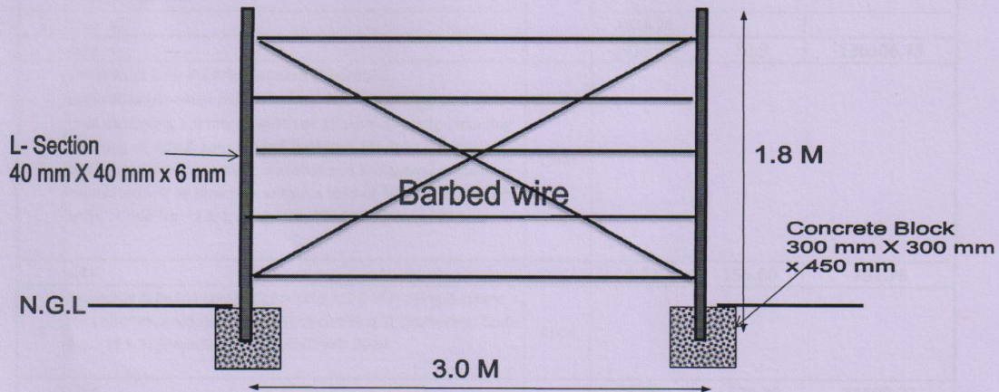
Drawing for Construction of Barbed wire Fencing 500 Mtrs
