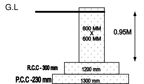
DETAILL OF COL. FOUND.
