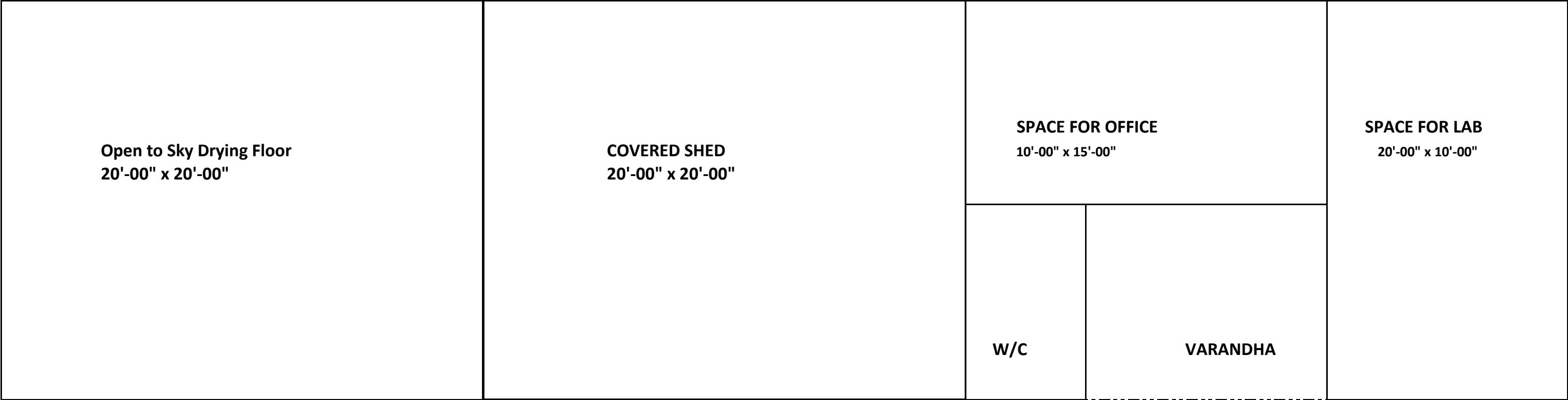
LAB./Office BLOCK 20'-00" x 25'-00"
