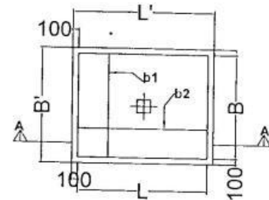
TYPICAL PLAN OF FOOTING READ ALONG WITH SCHEDULE
